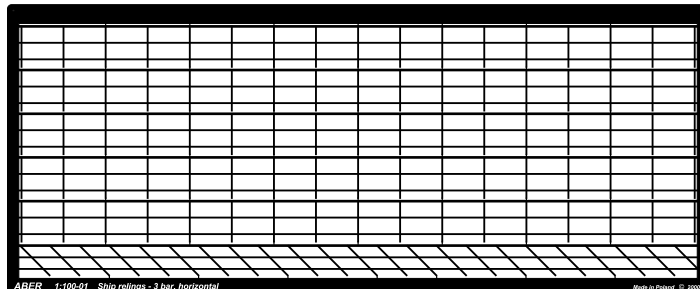
ABER 1:100-01 Ship railings - 3 bar, horizontal
